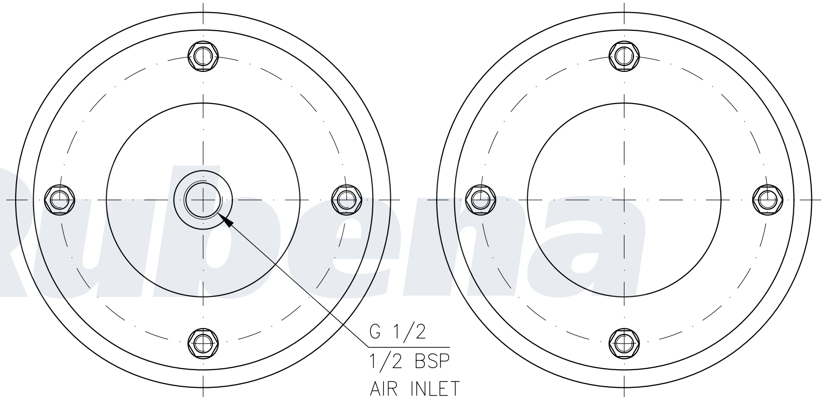
TOP VIEW
