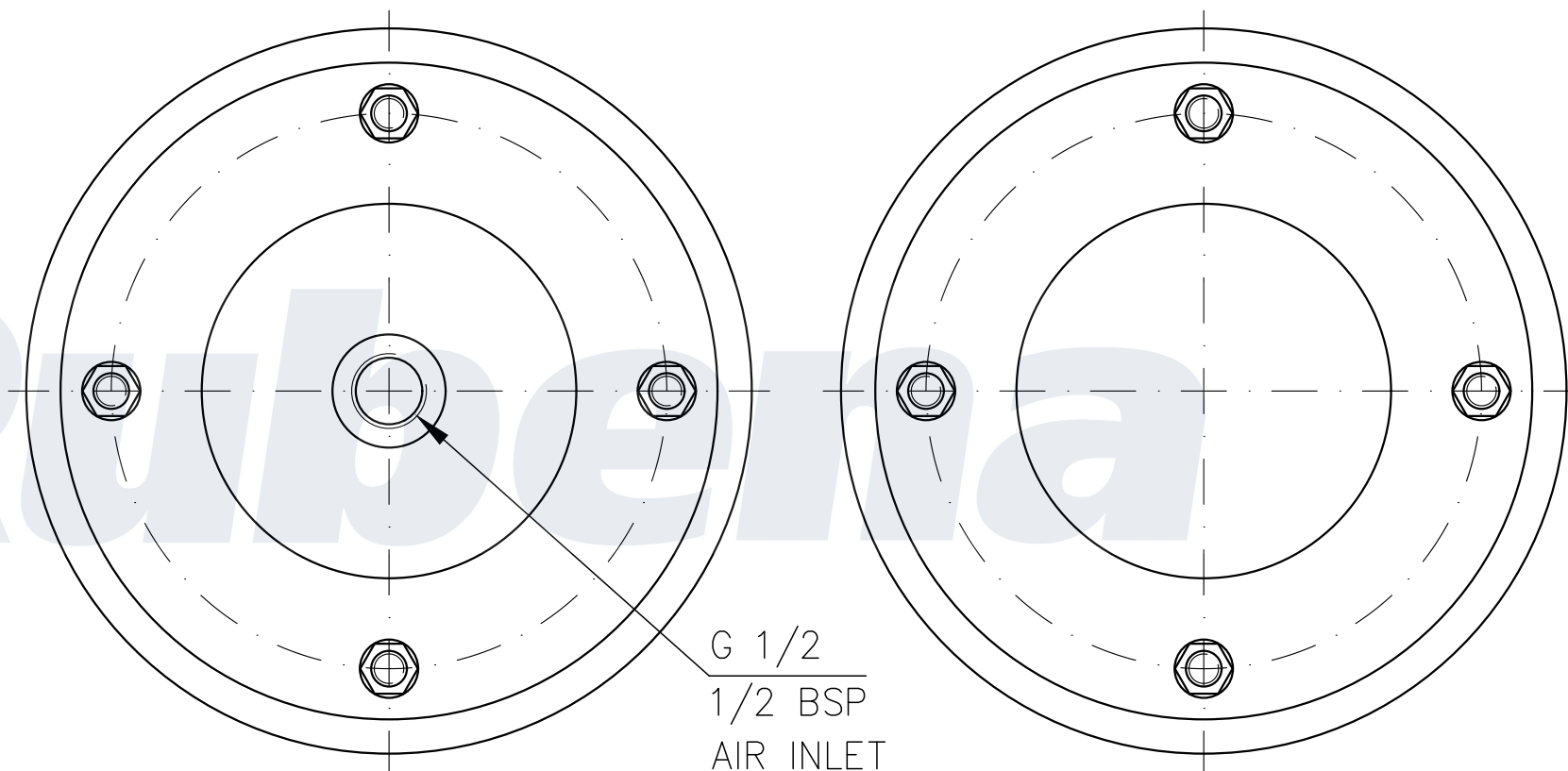
TOP VIEW
