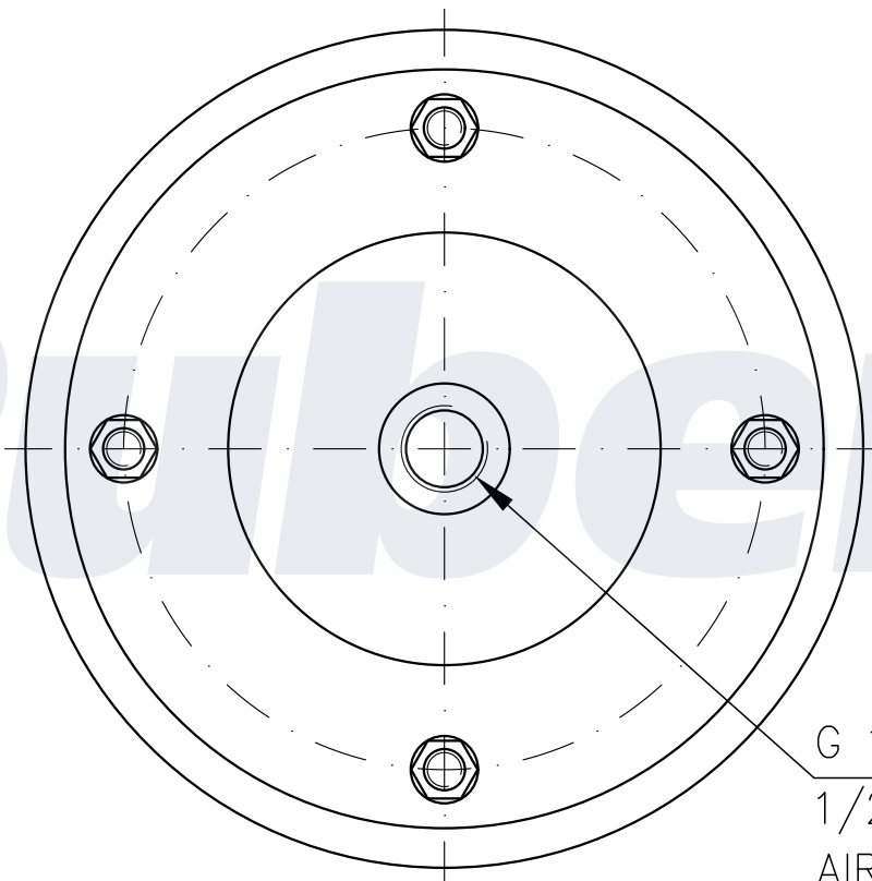
TOP VIEW
