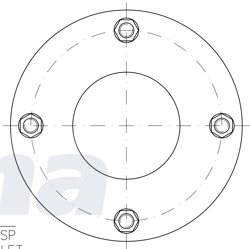
BOTTOM VIEW
