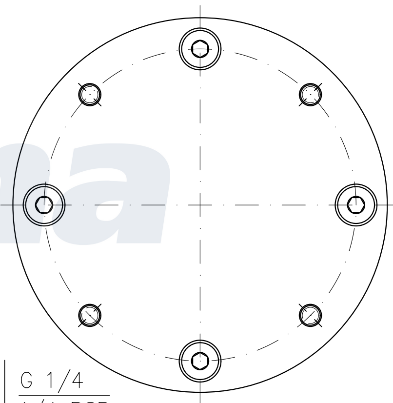
BOTTOM VIEW
