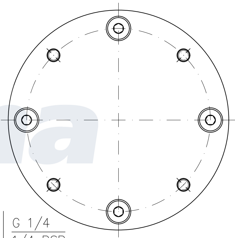
BOTTOM VIEW
