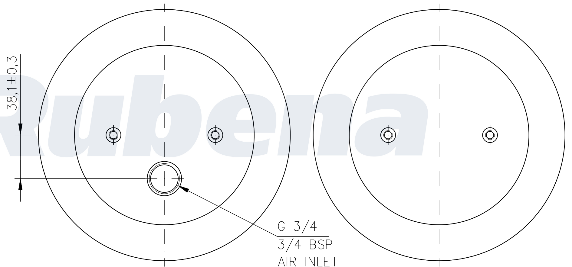
TOP VIEW
