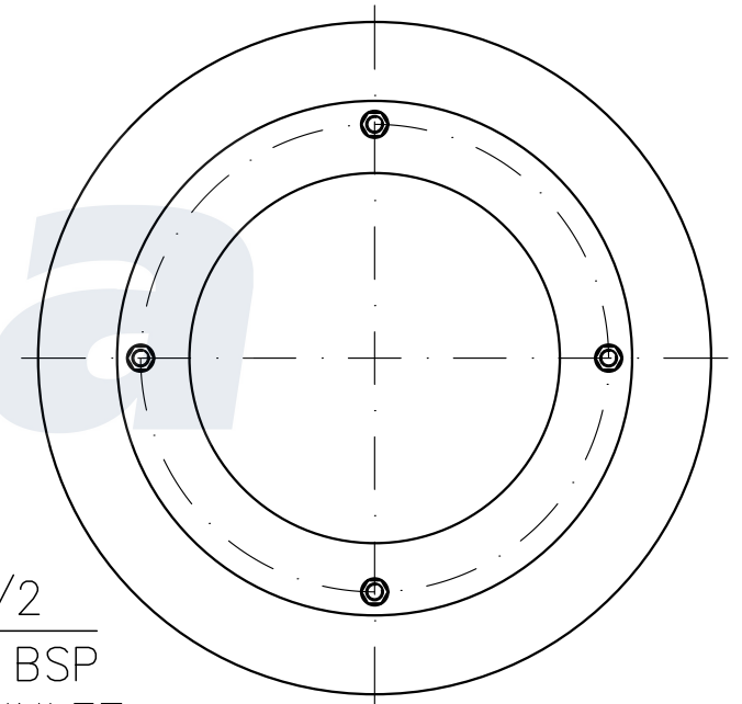
BOTTOM VIEW (1:2)
