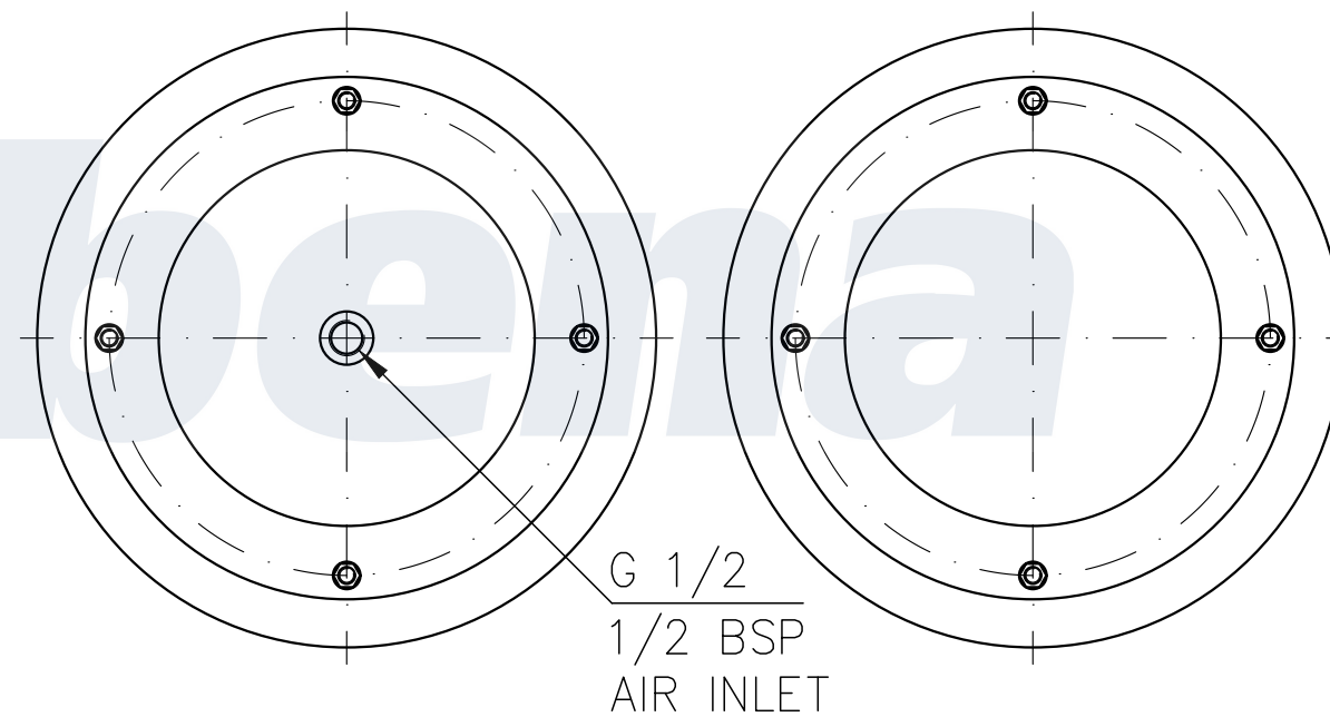
TOP VIEW (1:2)
