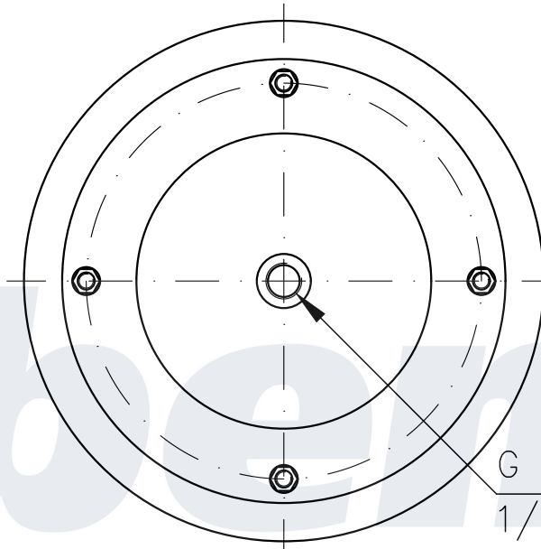
TOP VIEW (1:2)
