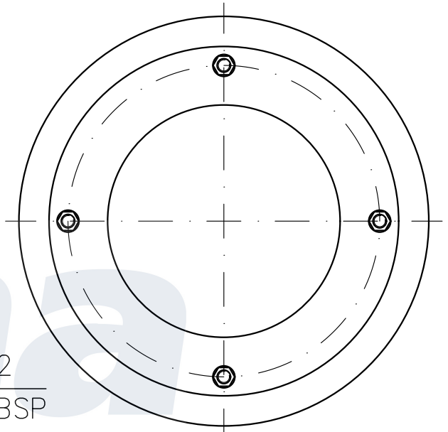
BOTTOM VIEW (1:2)
