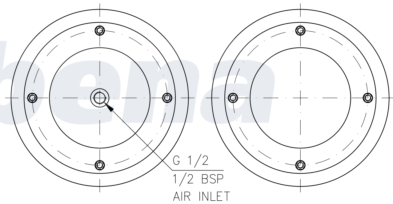
TOP VIEW (1:2)
