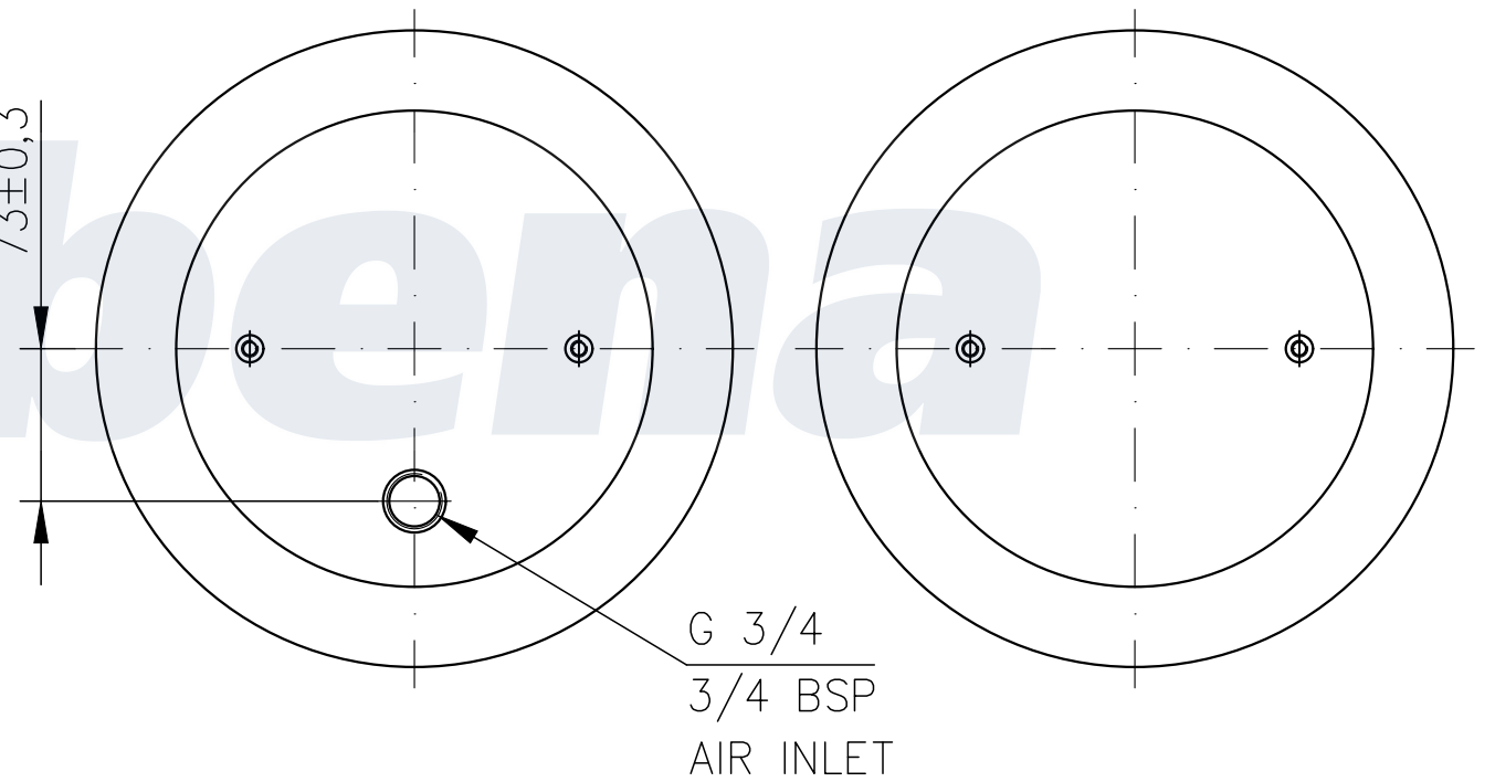
TOP VIEW (1:2)
