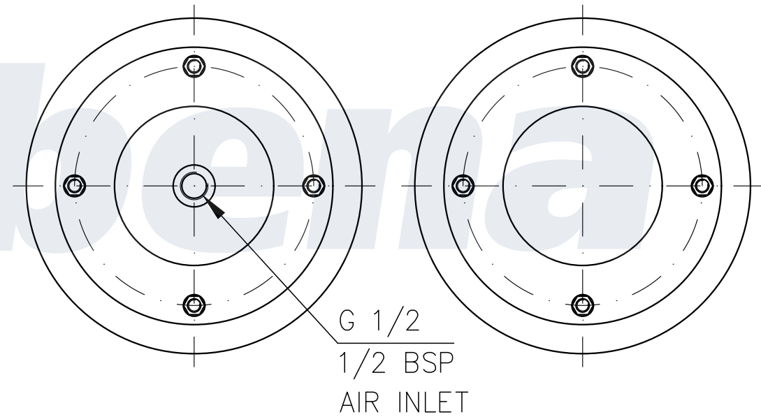
TOP VIEW (1:2)
