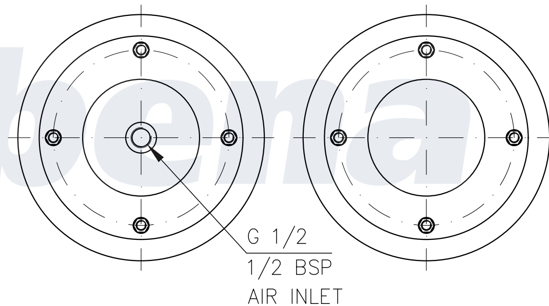
TOP VIEW (1:2)
