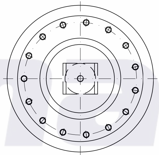
BOTTOM VIEW (1:2)
